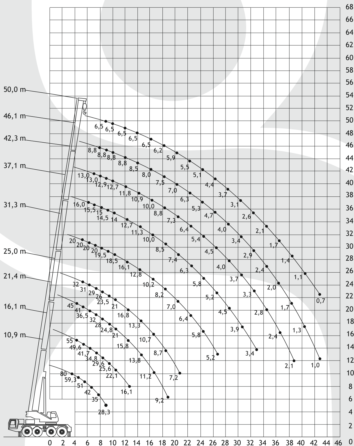
Working range: main boom
