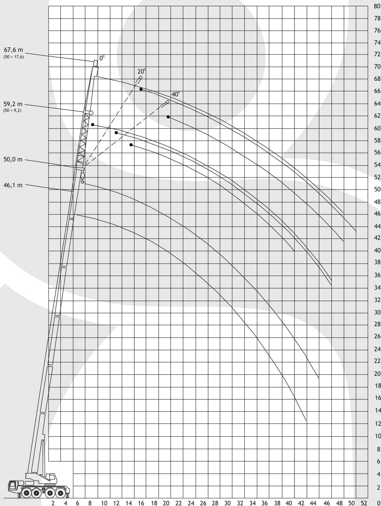
Working range: main boom + fix jib
